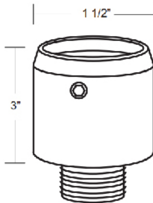
Dimensions: 1 1/2" dia. x 3" length
