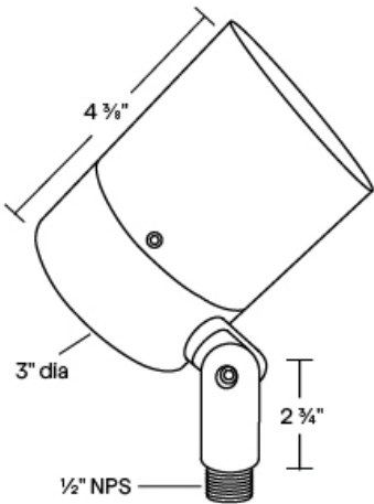
Weight: 2.1 lbs Dimensions: 3" dia. x 7" overall
