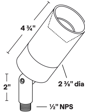
Dimensions: 2 3/8" dia. x 4 3/4"
