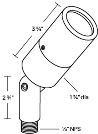
Dimensions: 1 3/4" dia. x 6" overall
