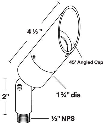
Dimensions: 1 3/4" dia. x 4 1/2"
