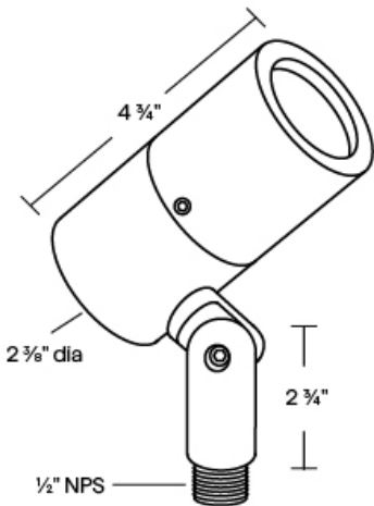
AL-1 Shown in Bronze Powder Coat Finish (BZ)Knuckle: Tapered & Positive Locking Weight: 1.6 lbsDimensions: 2 3/8" dia. x 4 3/4" overall
