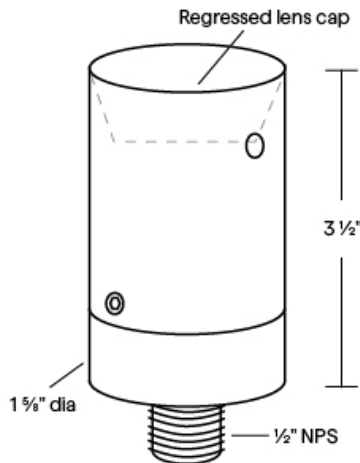
UD-2 Shown in Bronze Powder Coat Finish (BZ) Dimensions: 1 5/8" dia. x 3 1/2" overall
