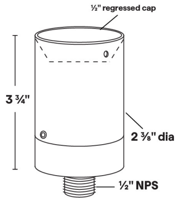
Dimensions: 2 3/8" dia. x 3 3/4"
