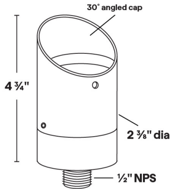
Dimensions: 2 3/8" dia. x 4 3/4"
