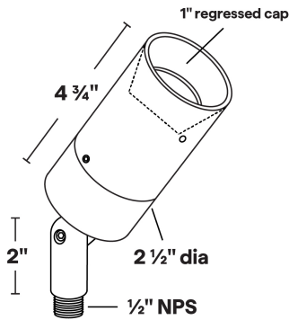
Dimensions: 2 1/2" dia x 4 3/4"
