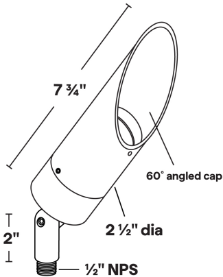
Dimensions: 2 1/2" dia. x 7 3/4"
