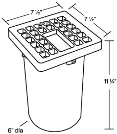
IN-15L Shown in Black Powder Coat Finish (BK) Dimensions: 7 1/2 " square x 11 1/4" high
