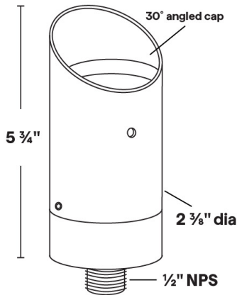
Dimensions: 2 3/8" dia. x 5 3/4"
