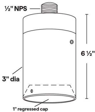
DL-29 Shown in Bronze Texture Powder Coat Finish (BZT) Dimensions: 3" dia. x 6 1/2"
