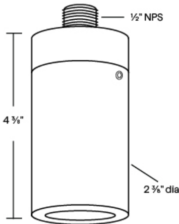
DL-10 Shown in Bronze Texture Powder Coat Finish Weight: Aluminum .8lbsOverall Dimensions: 2 3/8" dia. x 4 3/8" long
