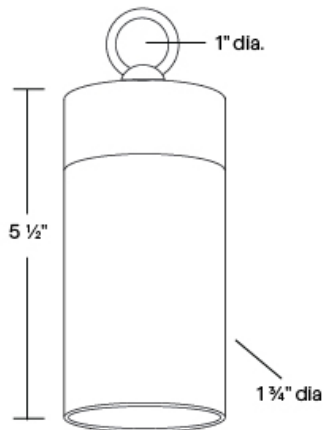
RL-3 Shown in Bronze Texture Powder Coat Finish (BZ) Overall Dimensions: 1 3/4" dia. x 5 1/2" overall
