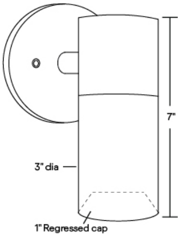
Weight:2.1 lbs Overall Dimensions: 3" dia. x 7" overall
