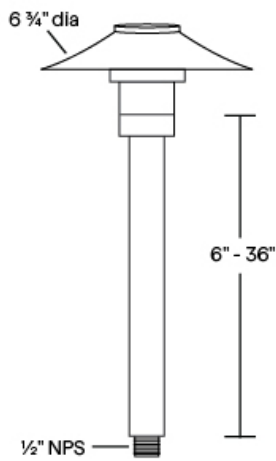
PL-1 Shown in Bronze Powder Coat Finish (BZ) Dimensions: Aluminum: 6 3/4" dia. shade, 1" dia. stem
