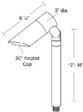
PL-12L Shown in Bronze Powder Coat Finish (BZ) Weight: 2.4 lbs. Overall Dimensions 3" dia. x 6 1/4" long
