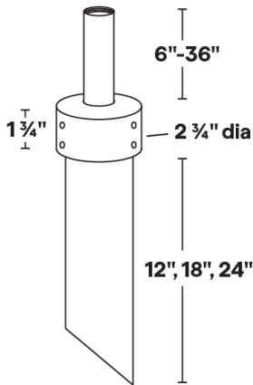
MT-2 Shown in Bronze Texture Powder Coat Finish (BZT) Dimensions: 2 3/4" dia. x 1 3/4" cap
