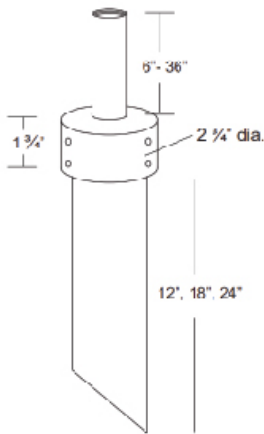
MT-2 Shown in Bronze Powder Coat Finish (BZ) Weight: 1.8 lbs.Dimensions: 2 3/4" dia. cap, 2 3/8" dia. stake
