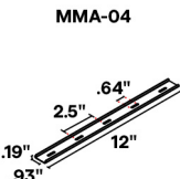
Magnet Mount Accessory for M4
