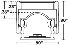
Profile with plastic louver
