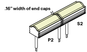
Continuous Bottom Feed
