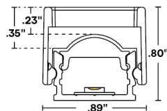
Profile with plastic louver
