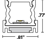
Profile with flat lens and low profile magnet
