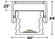
Profile with plastic louver
