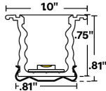
Profile with stainless steel mounting clip
