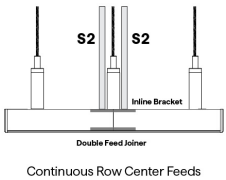
Continuous Row Center Feeds
