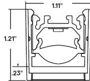
Profile with GZR & L1 Louver
