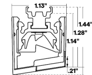
Profile with TBC-06 & L1 Louver
