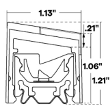
Profile with concealed clip & L1 Louver
