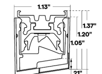
Profile with TBC-07 & L1 Louver
