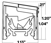
Profile with L1 Louver
