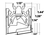
Profile with TBC-06 & L1 Louver
