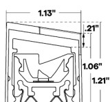
Profile with concealed clip & L1 Louver
