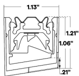
Profile with TBC-05 & L1 Louver
