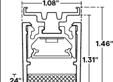
Profile with TBC-08 & L2 Louver
