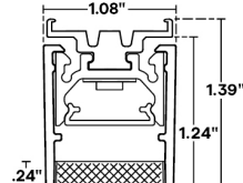
Profile with TBC-07 & L2 Louver
