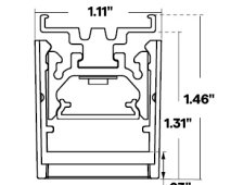
Profile with TBC-08 & L1 Louver
