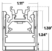
Profile with TBC-05 & L1 Louver
