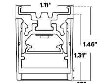
Profile with TBC-08 & L1 Louver
