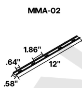
MMA-02 Magnet Mount Accessory for MG-02
