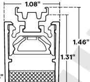
Profile with TBC-06 & L2 Louver
