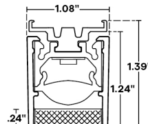
Profile with GRZ lens, TBC-07, & L2 Louver
