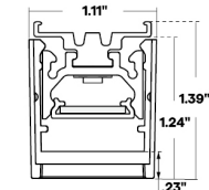
Profile with TBC-07 & L1 Louver
