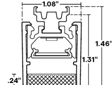
Profile with TBC-06 & L2 Louver
