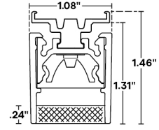
Profile with TBC-08 & L2 Louver
