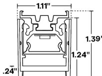
Profile with TBC-07 & louver
