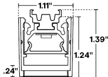
Profile with TBC-05 & louver
