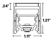
Profile with magnetic clip and louver
