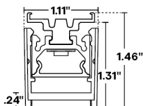
Profile with TBC-08 & louver
