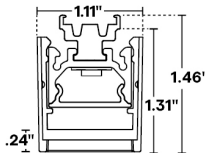
Profile with TBC-06 & louver
