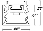
Profile with TBC-03
