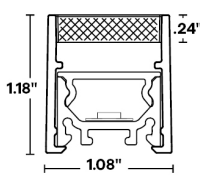
Profile with L2 Louver
