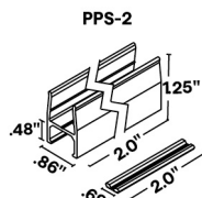
PVC Mounting Clip
